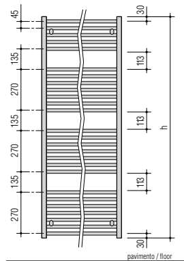
Mod. 150 - 26 tubi / tubes
