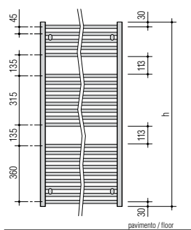
Mod. 120 - 22 tubi / tubes
