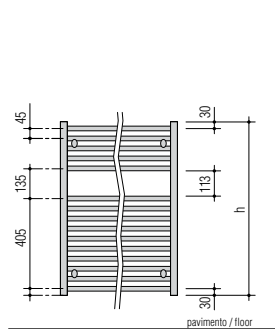
Mod. 80 - 15 tubi / tubes
