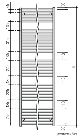
Mod. 180 - 31 tubi / tubes
