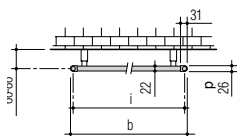
Mod. 80 - 15 tubi / tubes
