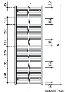
Mod. 150 - 26 Rohre / tubes
