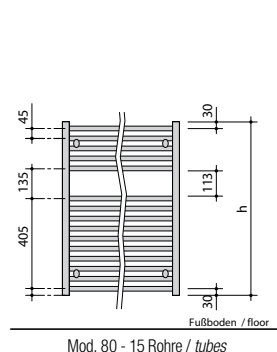
Mod. 80 - 15 Rohre / tubes
