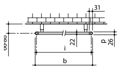
Mod. 80 - 15 Rohre / tubes
