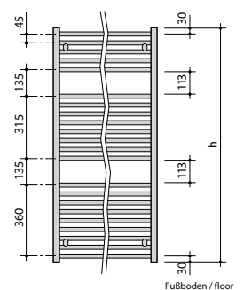
Mod. 120 - 22 Rohre / tubes
