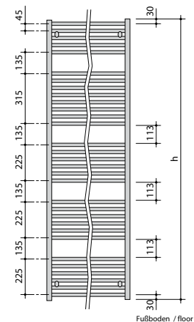
Mod. 180 - 31 Rohre / tubes
